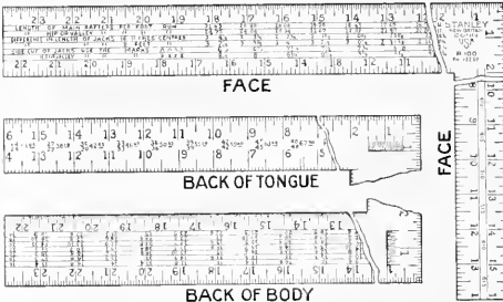
Stanley Steel Square.
